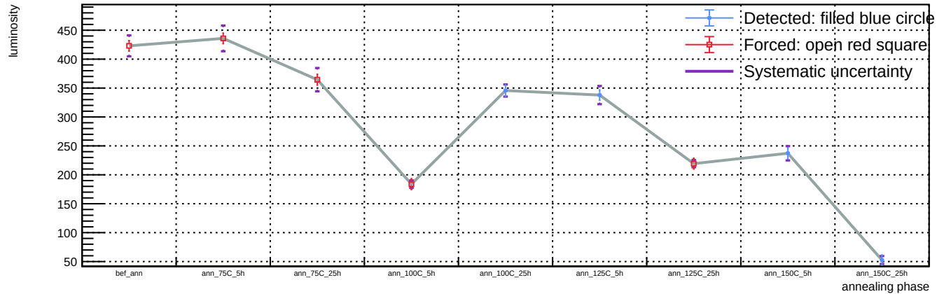
Sensor B1, T = 20 C, representative v = 55.9 V (max available) - Spot 91: luminosity vs phase
