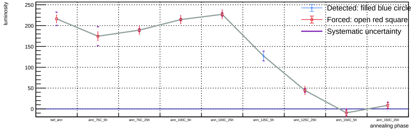
Sensor B1, T = 20 C, representative v = 55.9 V (max available) - Spot 95: luminosity vs phase
