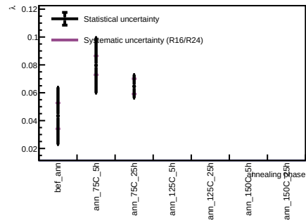
Sensor B1, v = 3 V - Spot 2
