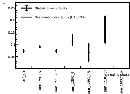
Sensor B1, v = 3 V - Spot 0
