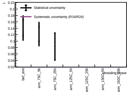
Sensor B1, v = 3 V - Spot 3
