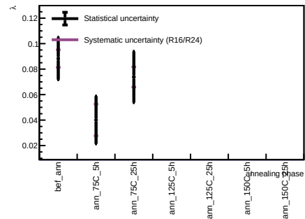
Sensor B1, v = 3 V - Spot 4
