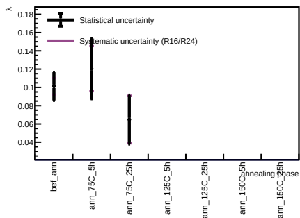
Sensor B1, v = 3 V - Spot 13
