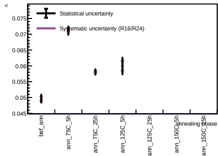
Sensor B1, v = 3 V - Spot 25
