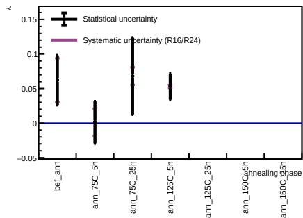
Sensor B1, v = 3 V - Spot 28
