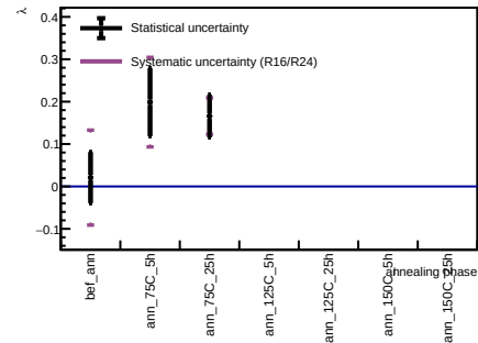
Sensor B1, v = 3 V - Spot 47
