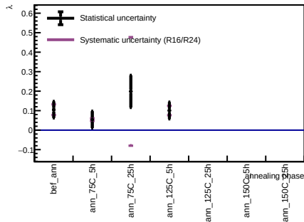
Sensor B1, v = 3 V - Spot 46
