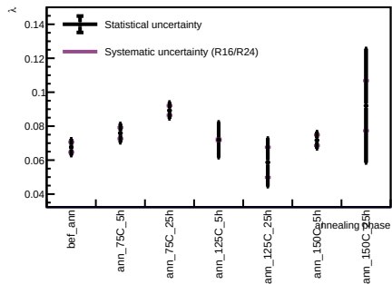
Sensor B1, v = 3 V - Spot 60
