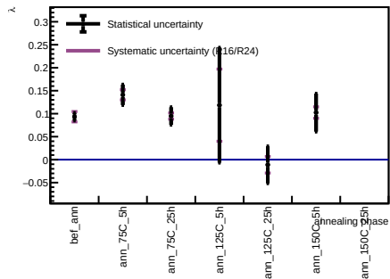
Sensor B1, v = 3 V - Spot 61
