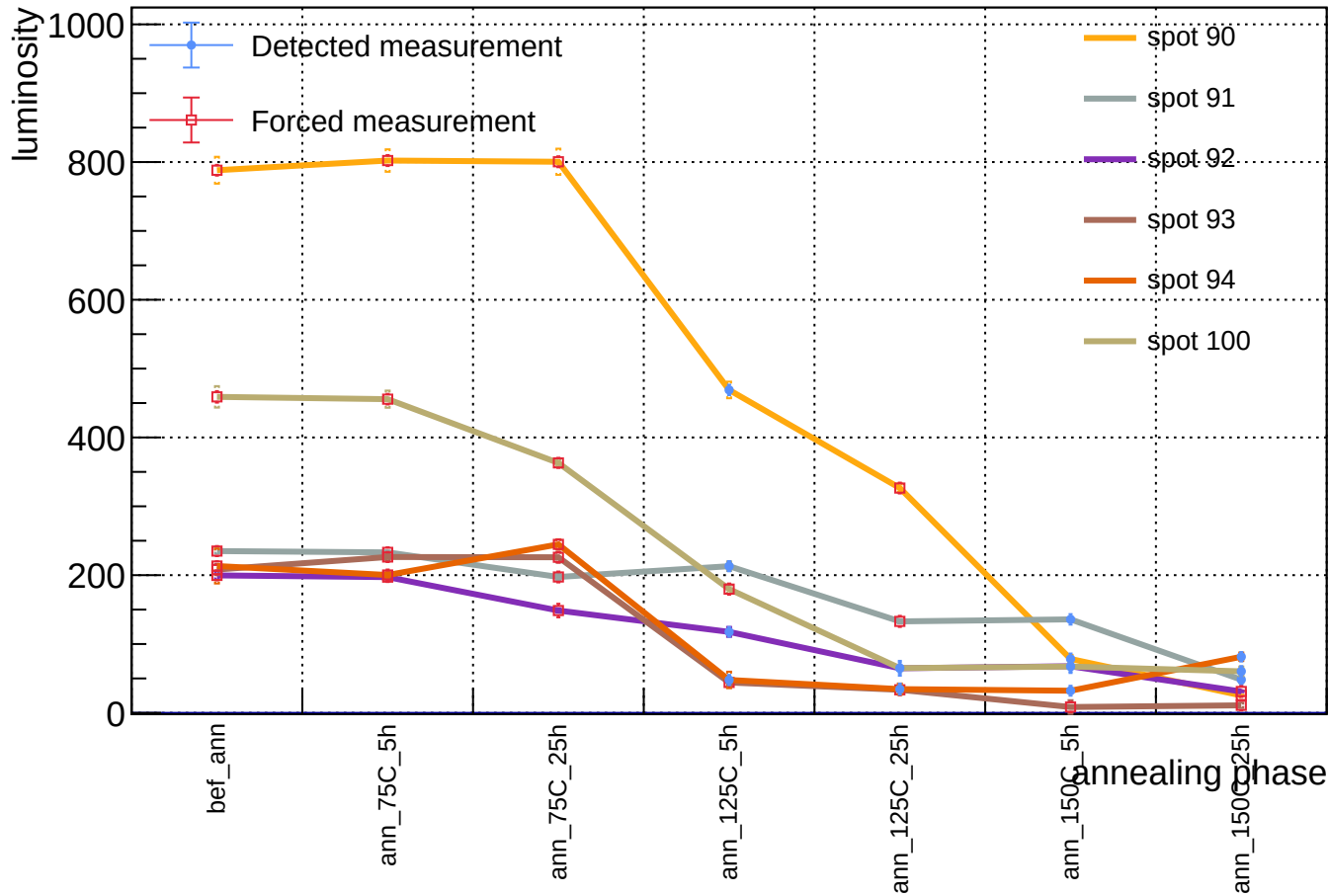
Sensor B1, v = 3 V, representative T = 23 C (max available) - luminosity vs phase - order 10^2
