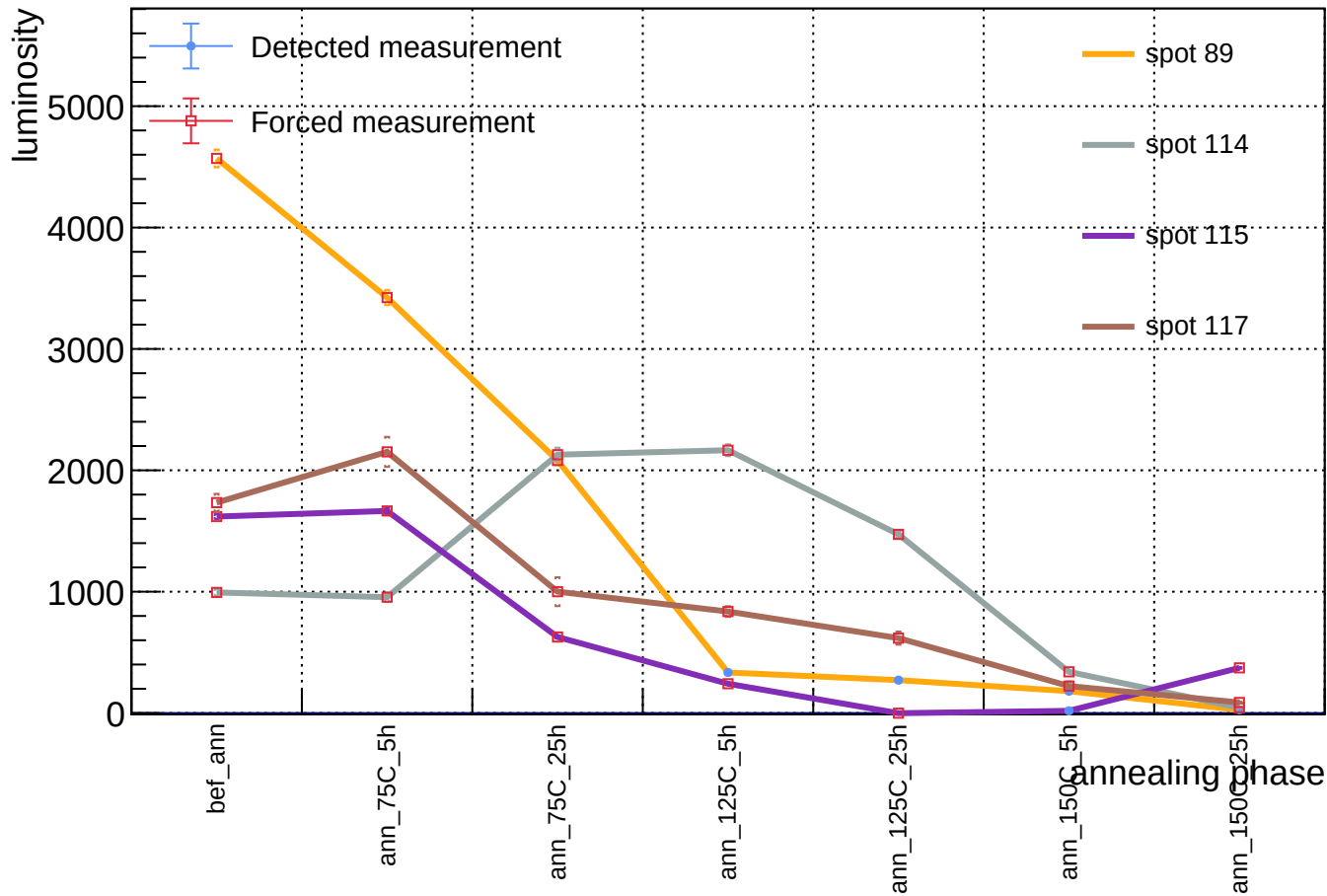
Sensor B1, v = 3 V, representative T = 23 C (max available) - luminosity vs phase - order 10^3
