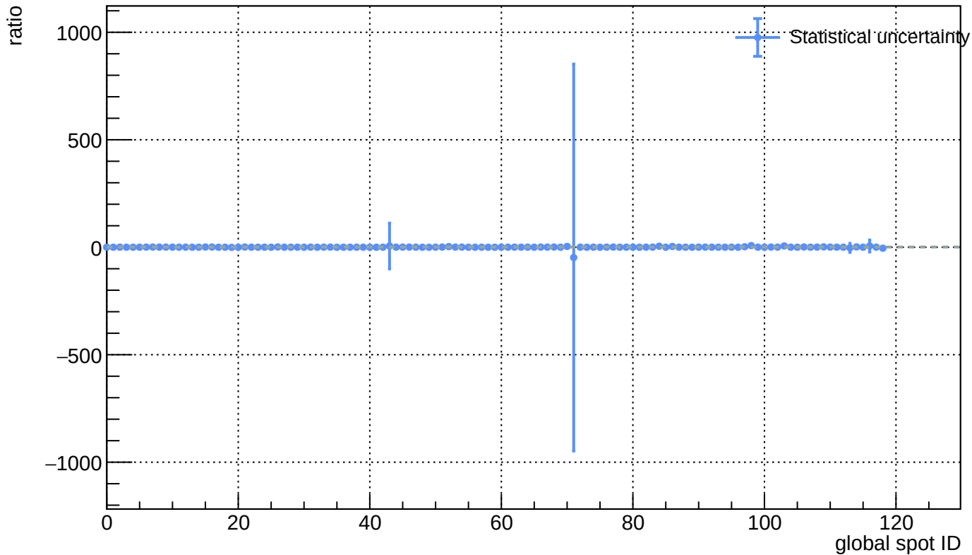
Sensor B1, v = 3 \text{ V} - L(\text{ann\_125C\_25h}) / L(\text{before\_annealing})
