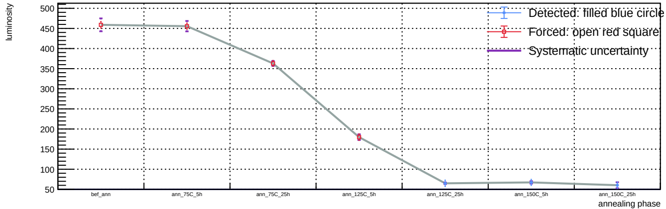
Sensor B1, v = 3 V, representative T = 23 C (max available) - Spot 100: luminosity vs phase
