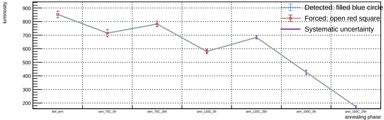
Sensor B1, v = 3 V, representative T = 23 C (max available) - Spot 101: luminosity vs phase
