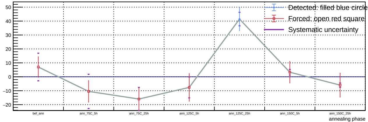
Sensor B1, v = 3 V, representative T = 23 C (max available) - Spot 103: luminosity vs phase
