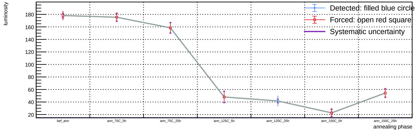
Sensor B1, v = 3 V, representative T = 23 C (max available) - Spot 104: luminosity vs phase
