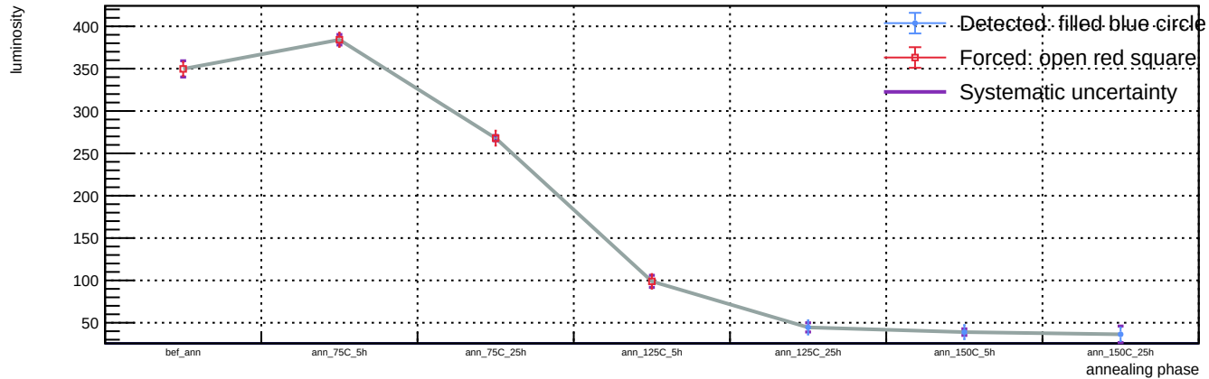
Sensor B1, v = 3 V, representative T = 23 C (max available) - Spot 105: luminosity vs phase
