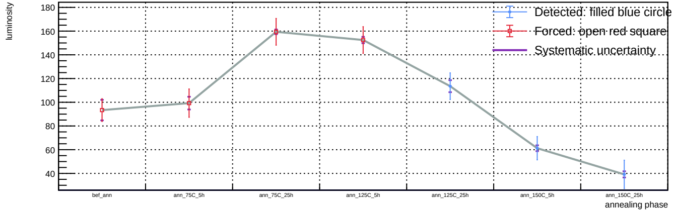
Sensor B1, v = 3 V, representative T = 23 C (max available) - Spot 106: luminosity vs phase
