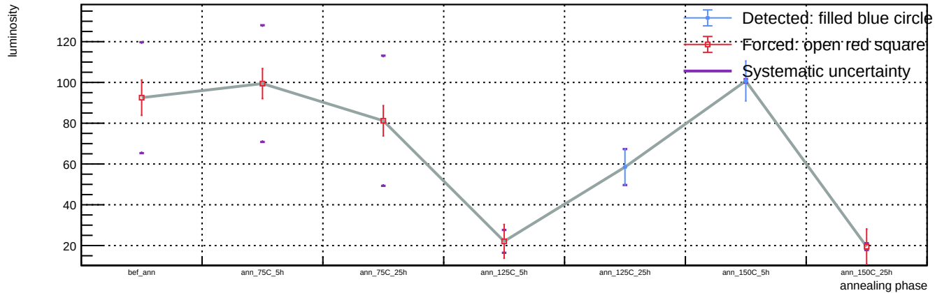
Sensor B1, v = 3 V, representative T = 23 C (max available) - Spot 108: luminosity vs phase
