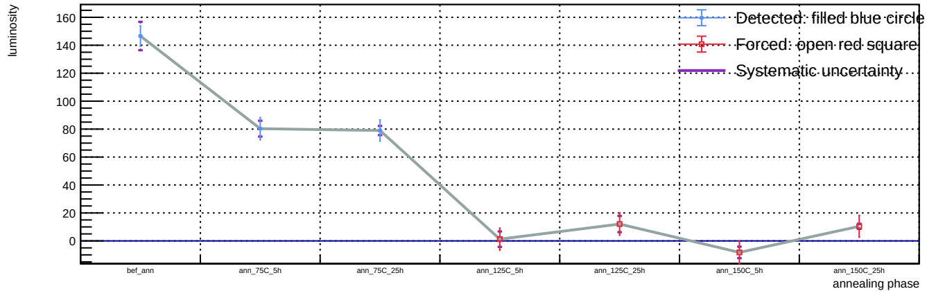
Sensor B1, v = 3 V, representative T = 23 C (max available) - Spot 13: luminosity vs phase
