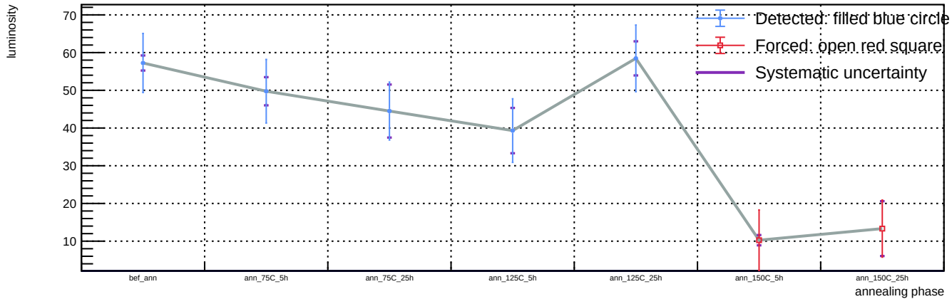
Sensor B1, v = 3 V, representative T = 23 C (max available) - Spot 15: luminosity vs phase
