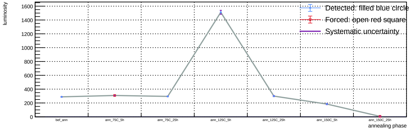
Sensor B1, v = 3 V, representative T = 23 C (max available) - Spot 16: luminosity vs phase
