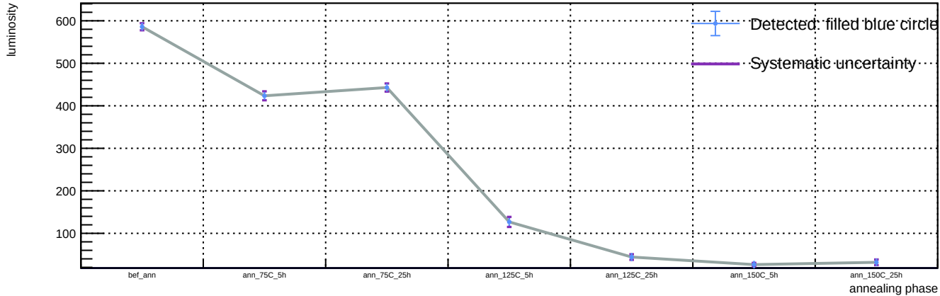
Sensor B1, v = 3 V, representative T = 23 C (max available) - Spot 18: luminosity vs phase
