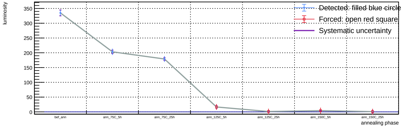
Sensor B1, v = 3 V, representative T = 23 C (max available) - Spot 20: luminosity vs phase
