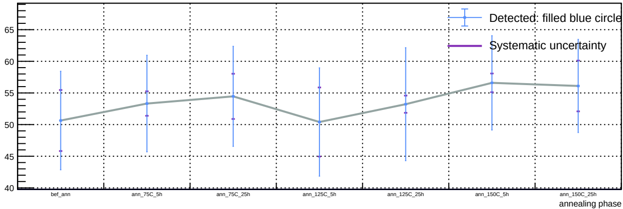
Sensor B1, v = 3 V, representative T = 23 C (max available) - Spot 21: luminosity vs phase
