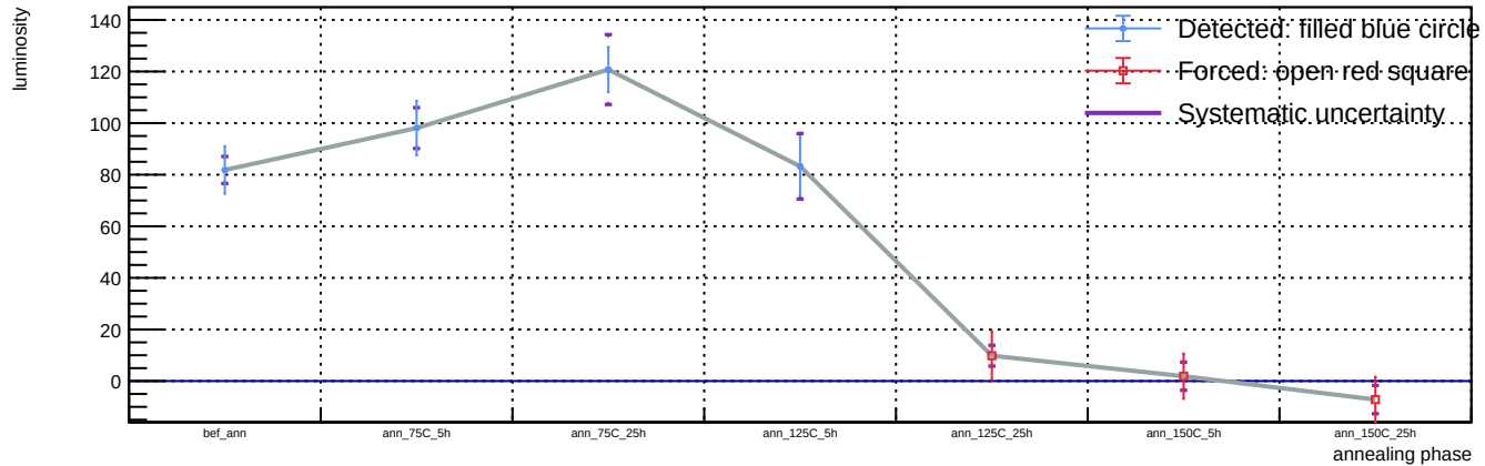
Sensor B1, v = 3 V, representative T = 23 C (max available) - Spot 22: luminosity vs phase
