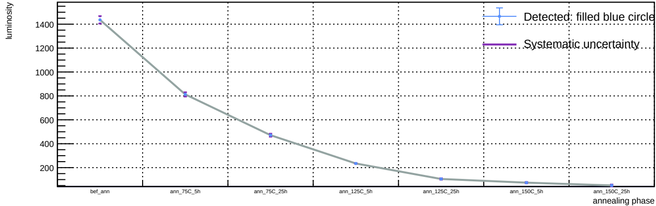
Sensor B1, v = 3 V, representative T = 23 C (max available) - Spot 23: luminosity vs phase
