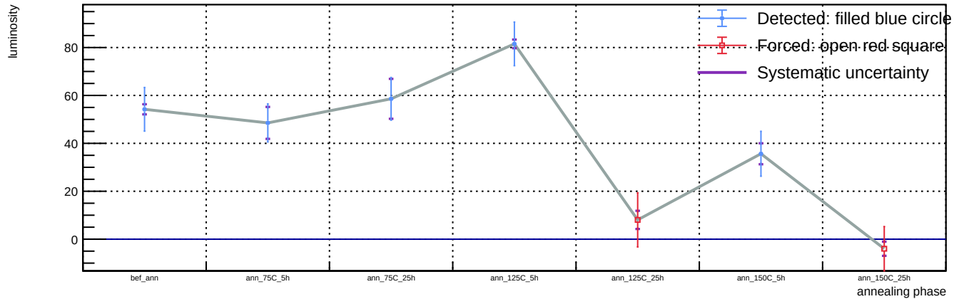
Sensor B1, v = 3 V, representative T = 23 C (max available) - Spot 27: luminosity vs phase
