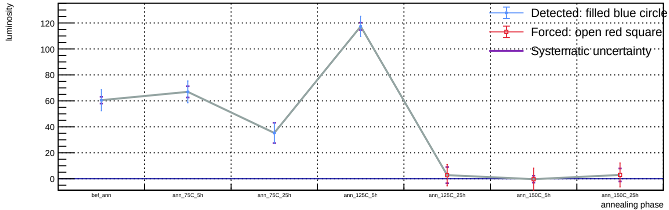
Sensor B1, v = 3 V, representative T = 23 C (max available) - Spot 28: luminosity vs phase
