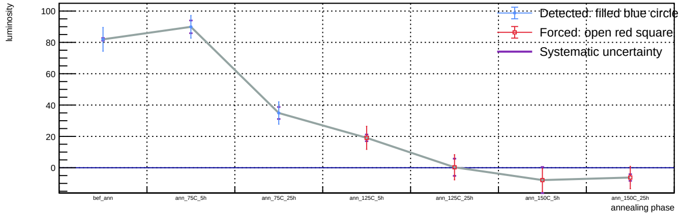
Sensor B1, v = 3 V, representative T = 23 C (max available) - Spot 32: luminosity vs phase
