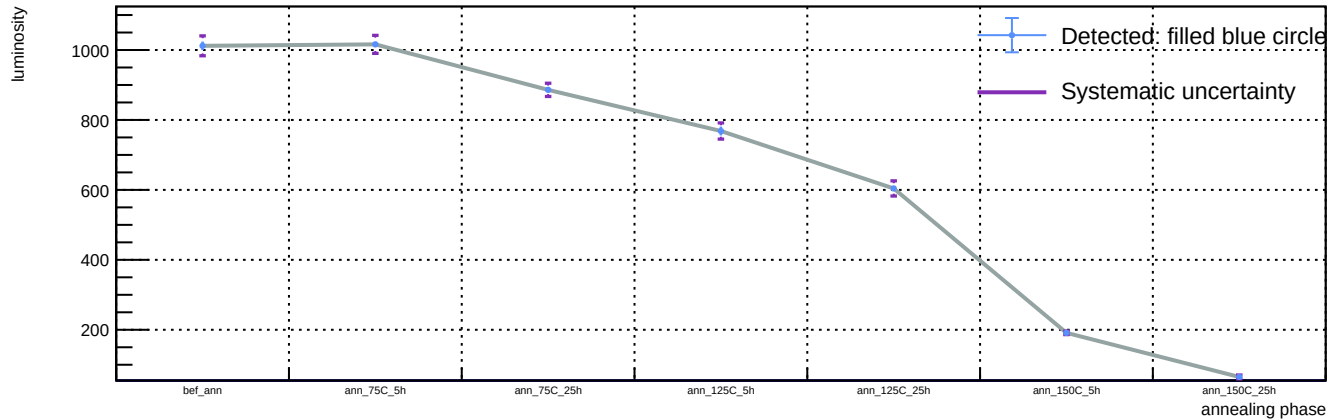
Sensor B1, v = 3 V, representative T = 23 C (max available) - Spot 34: luminosity vs phase
