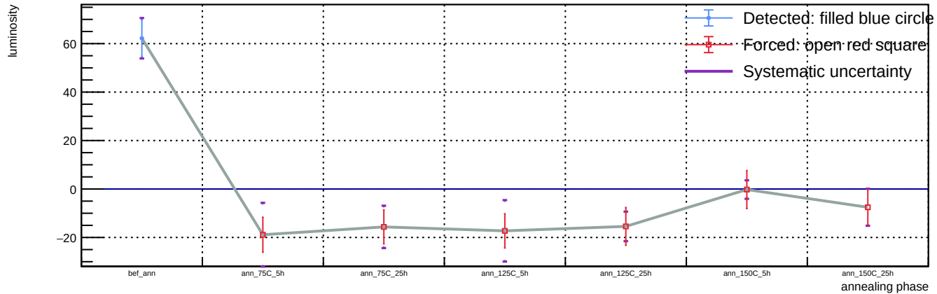
Sensor B1, v = 3 V, representative T = 23 C (max available) - Spot 35: luminosity vs phase
