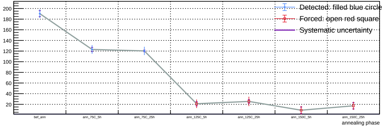
Sensor B1, v = 3 V, representative T = 23 C (max available) - Spot 39: luminosity vs phase
