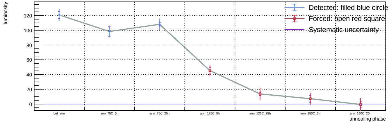
Sensor B1, v = 3 V, representative T = 23 C (max available) - Spot 4: luminosity vs phase
