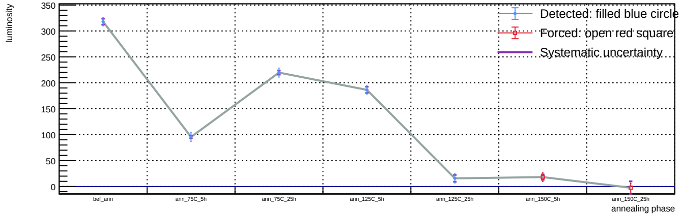
Sensor B1, v = 3 V, representative T = 23 C (max available) - Spot 40: luminosity vs phase
