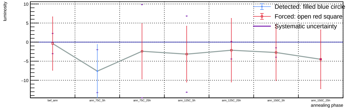
Sensor B1, v = 3 V, representative T = 23 C (max available) - Spot 43: luminosity vs phase
