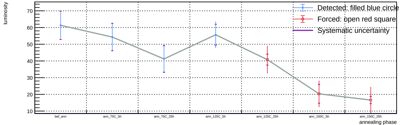
Sensor B1, v = 3 V, representative T = 23 C (max available) - Spot 46: luminosity vs phase
