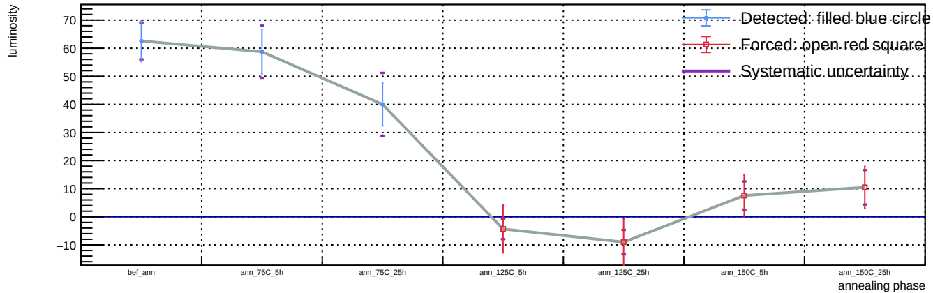
Sensor B1, v = 3 V, representative T = 23 C (max available) - Spot 49: luminosity vs phase
