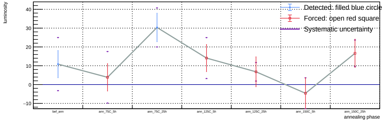
Sensor B1, v = 3 V, representative T = 23 C (max available) - Spot 54: luminosity vs phase
