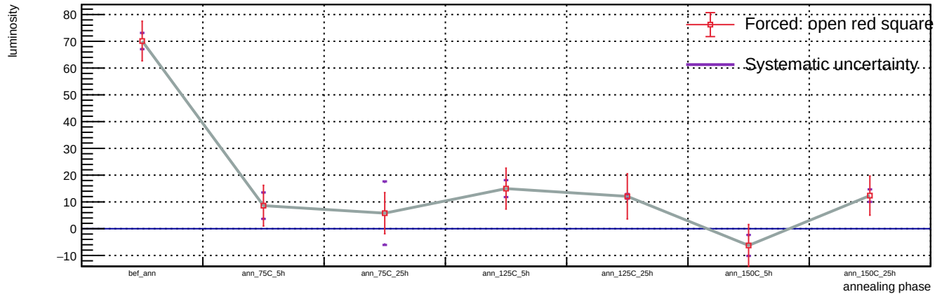
Sensor B1, v = 3 V, representative T = 23 C (max available) - Spot 57: luminosity vs phase
