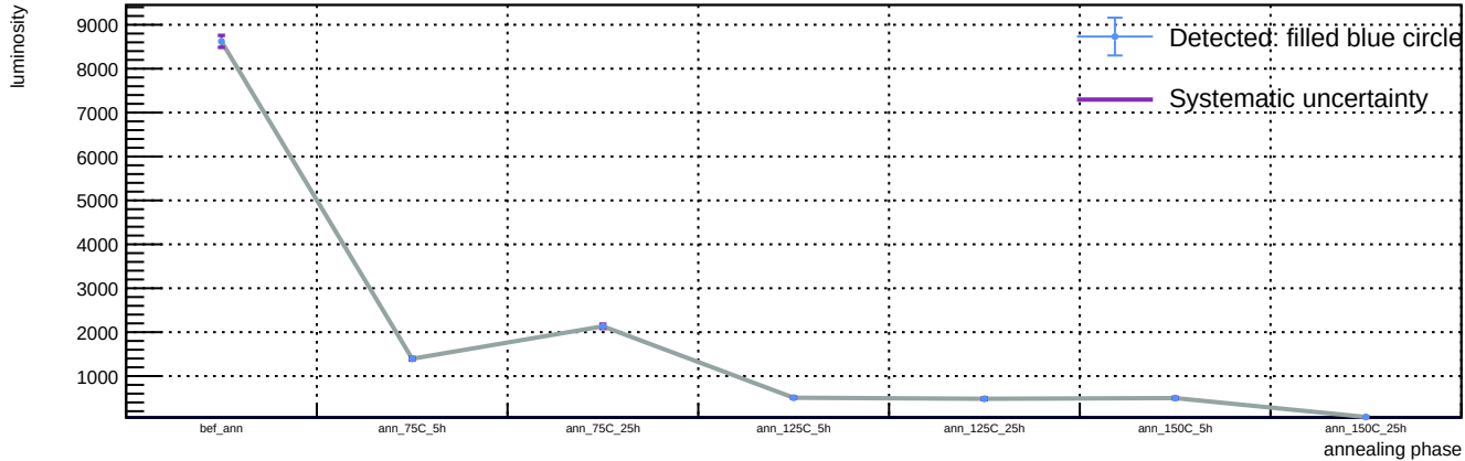
Sensor B1, v = 3 V, representative T = 23 C (max available) - Spot 65: luminosity vs phase
