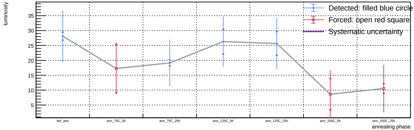
Sensor B1, v = 3 V, representative T = 23 C (max available) - Spot 68: luminosity vs phase
