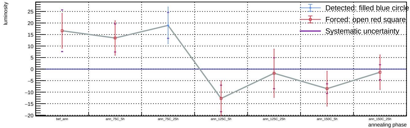
Sensor B1, v = 3 V, representative T = 23 C (max available) - Spot 75: luminosity vs phase
