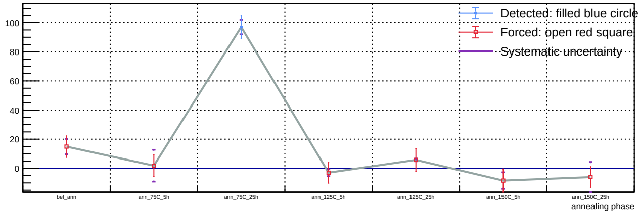
Sensor B1, v = 3 V, representative T = 23 C (max available) - Spot 76: luminosity vs phase
