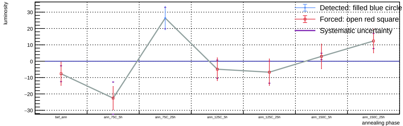
Sensor B1, v = 3 V, representative T = 23 C (max available) - Spot 77: luminosity vs phase
