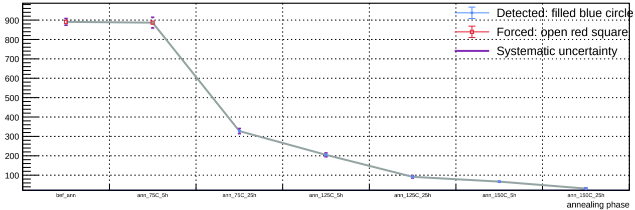
Sensor B1, v = 3 V, representative T = 23 C (max available) - Spot 78: luminosity vs phase
