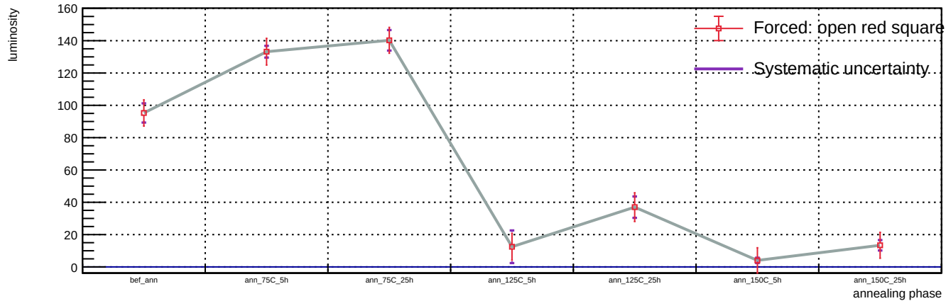
Sensor B1, v = 3 V, representative T = 23 C (max available) - Spot 80: luminosity vs phase
