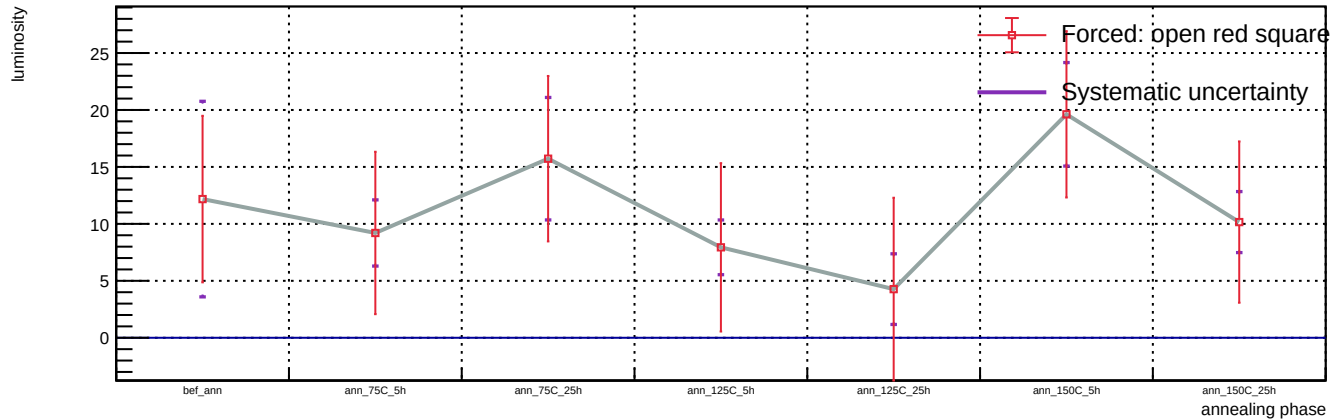
Sensor B1, v = 3 V, representative T = 23 C (max available) - Spot 82: luminosity vs phase
