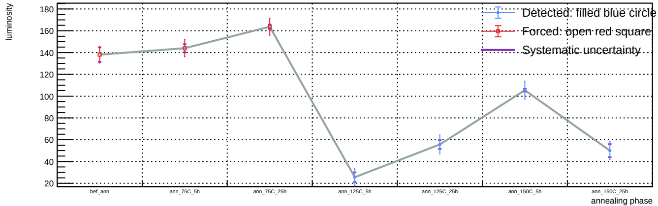
Sensor B1, v = 3 V, representative T = 23 C (max available) - Spot 83: luminosity vs phase
