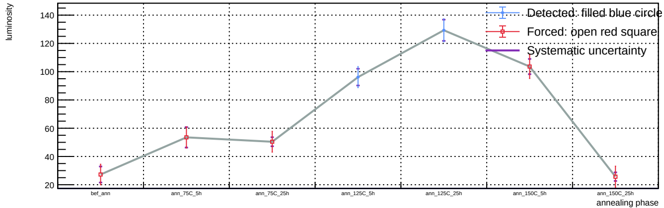
Sensor B1, v = 3 V, representative T = 23 C (max available) - Spot 84: luminosity vs phase
