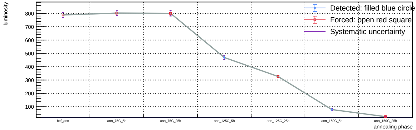
Sensor B1, v = 3 V, representative T = 23 C (max available) - Spot 90: luminosity vs phase
