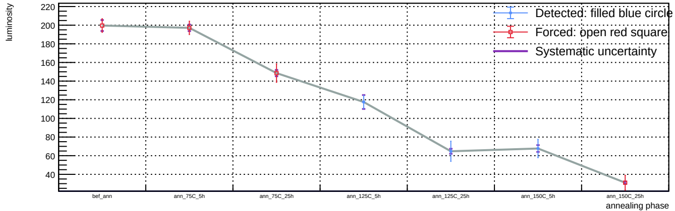
Sensor B1, v = 3 V, representative T = 23 C (max available) - Spot 92: luminosity vs phase
